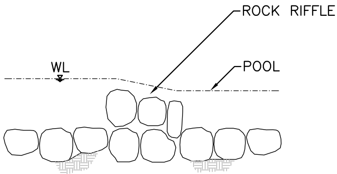
SECTION A BOAT/FISH BYPASS SCALE 1 INCH = 10 FEET
