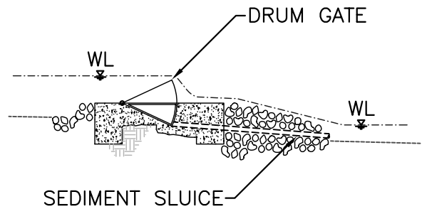
SECTION B DRUM GATE SPILLWAY SCALE 1 INCH = 10 FEET
